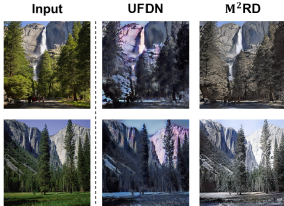
Fig. 5. Example results of the comparison with UFDN [26] in summer-to-winter translation. Note that since UFDN [26] does not observe and exhibit intra-domain image variety, its output might be irrational in terms of appearance or lighting (e.g., mix of daytime and nighttime appearance), while ours are more realistic and have a higher visual quality.
