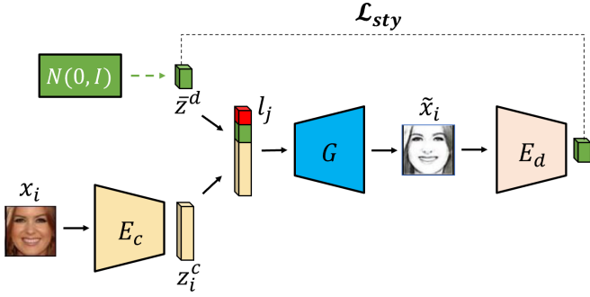
Fig. 3. In addition to the architecture described in Fig. 2, we further apply the objective function \mathcal{L}_{sty} to enforce the reconstruction on the domain-specific feature. More details can be found in Section III-C
