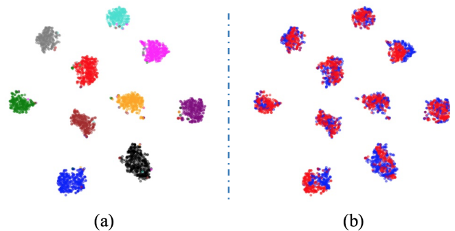
Fig. 12. t-SNE visualization of the handwritten digit data for USPS \rightarrow MNIST. Note that different colors indicate data of (a) different digits classes 0-9 and (b) different domains (source/target).
