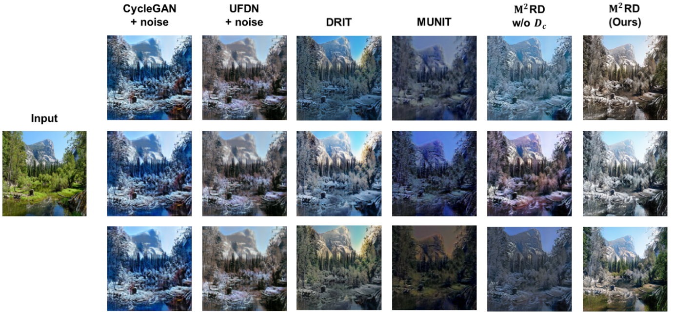
Fig. 4. Example results of our multi-modal image translations and the comparison with the existing image-to-image translation methods. We observe that our model is able to generate high-quality images with meaningful diversity.
