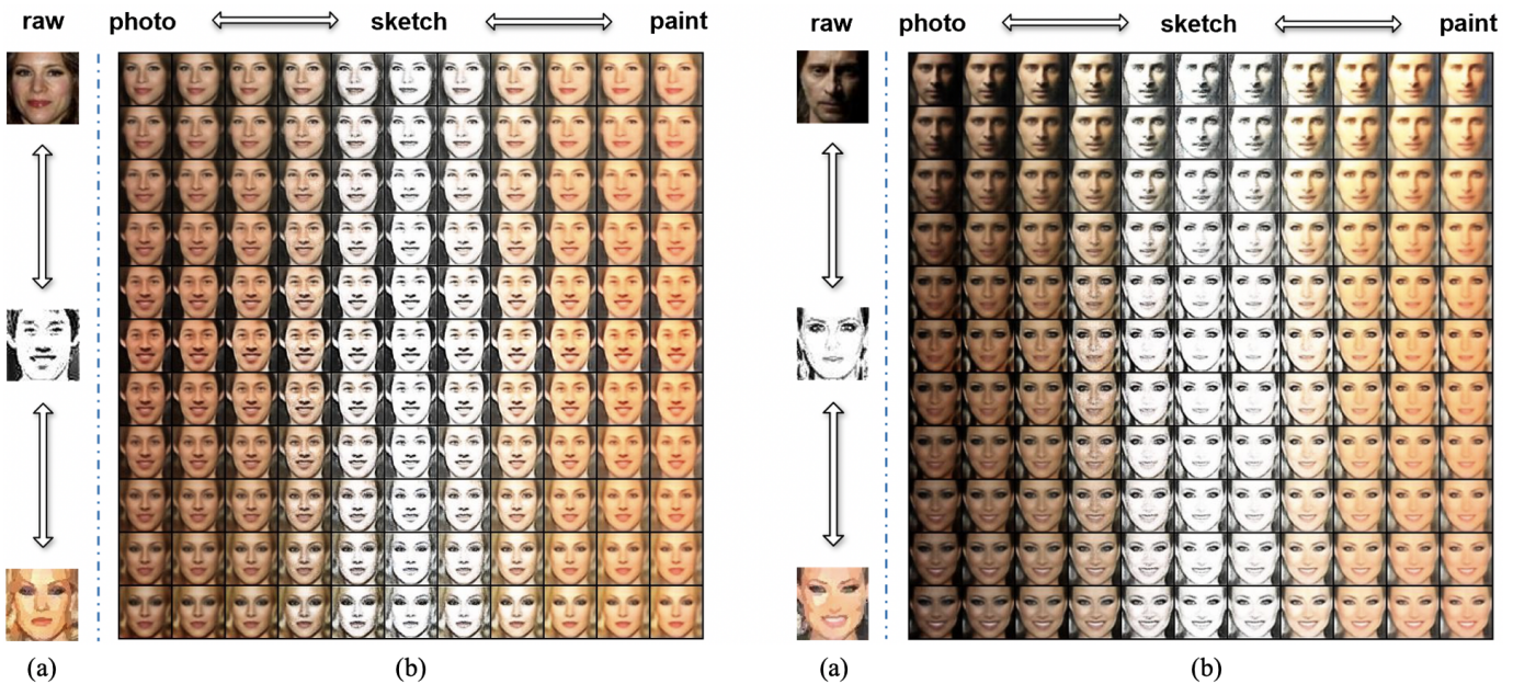
Fig. 7. Example results of image translation across multiple domains among photo/sketch/paint .
